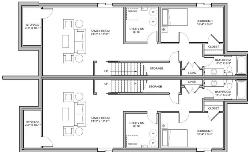
1 BASEMENT PLAN SCALE: 3/16" = 1'-0"
