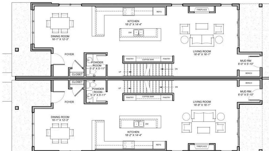
1 1ST FLOOR SCALE: 3/16" = 1'-0"
