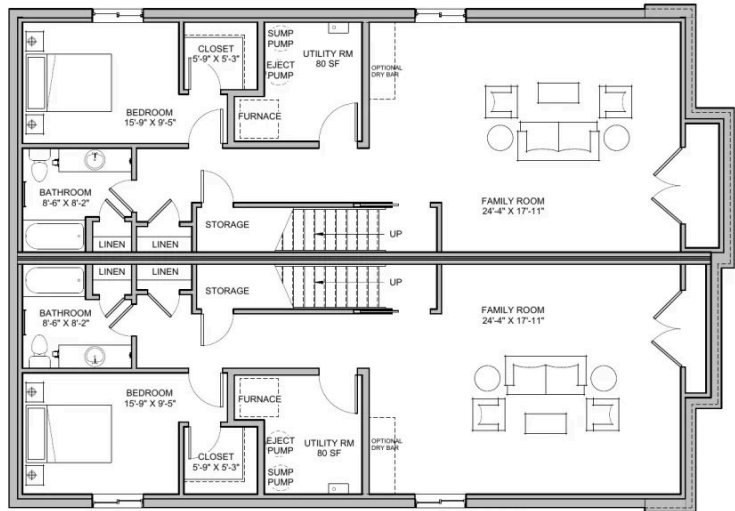
1 BASEMENT PLAN SCALE: 3/16" = 1'-0"
