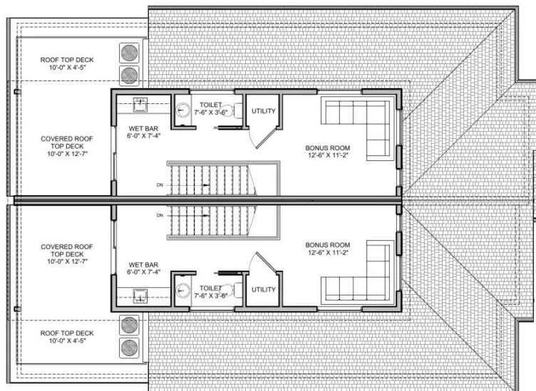
1 THIRD FLOOR PLAN - OPTION 1 SCALE: 3/16" = 1'-0"
