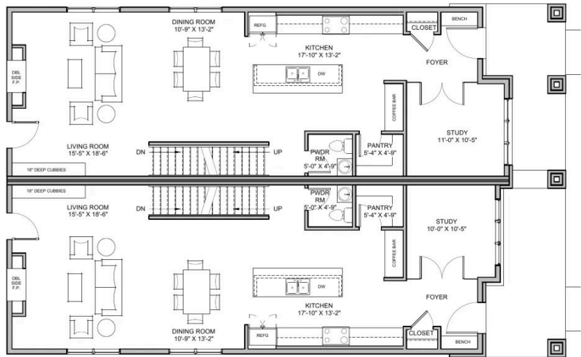
1 FIRST FLOOR PLAN SCALE: 3/16" = 1'-0"
