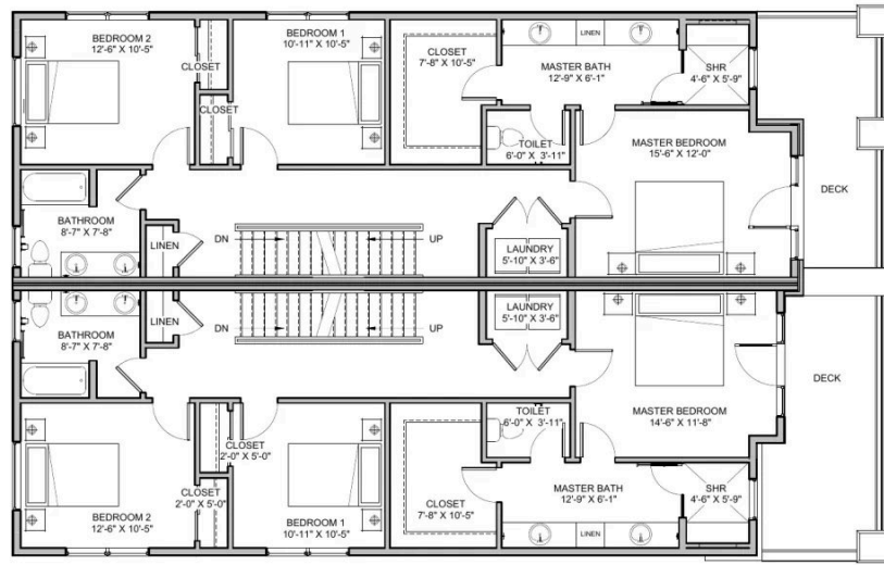
1 SECOND FLOOR PLAN SCALE: 3/16" = 1'-0"
