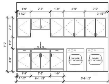
1 LAUNDRY ROOM SCALE: 3/8" = 1'-0"
