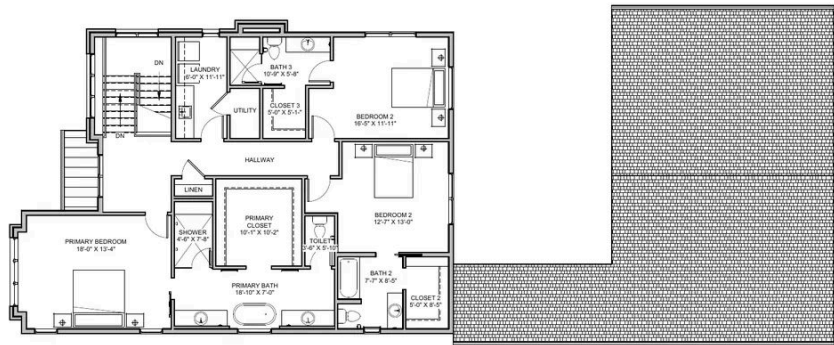
1 2ND FLOOR PLAN
